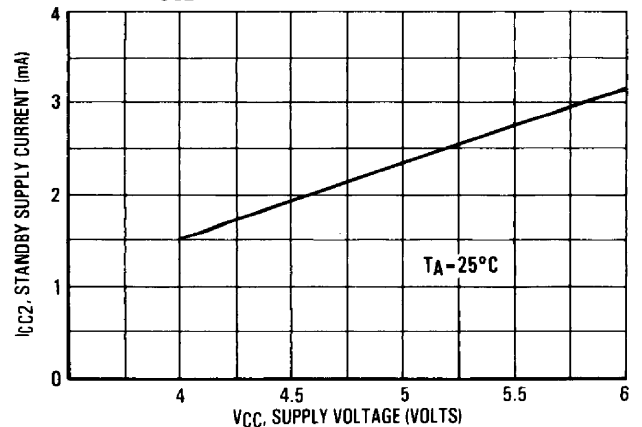
FIGURE 13 — I_{CC2} SUPPLY CURRENT versus SUPPLY VOLTAGE
