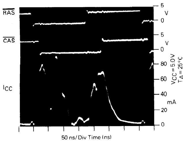
FIGURE 20 — \overline{\text{RAS}}/\overline{\text{CAS}} CYCLE
