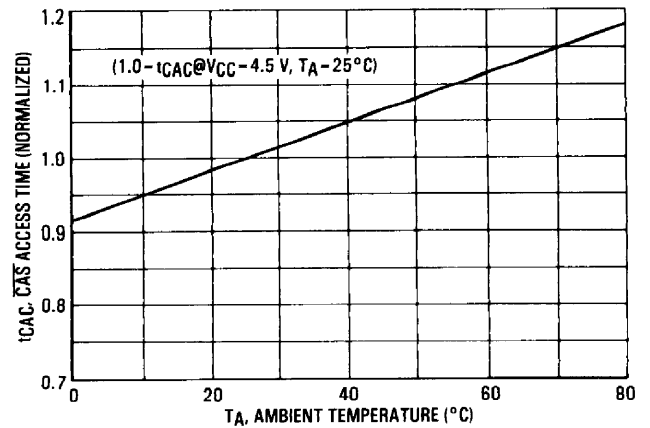
FIGURE 5 — \overline{\text{CAS}} ACCESS TIME versus AMBIENT TEMPERATURE
