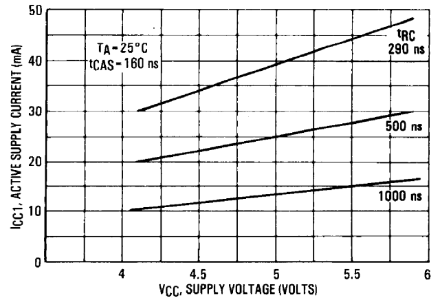
FIGURE 9 — I_{CC1} SUPPLY CURRENT versus SUPPLY VOLTAGE
