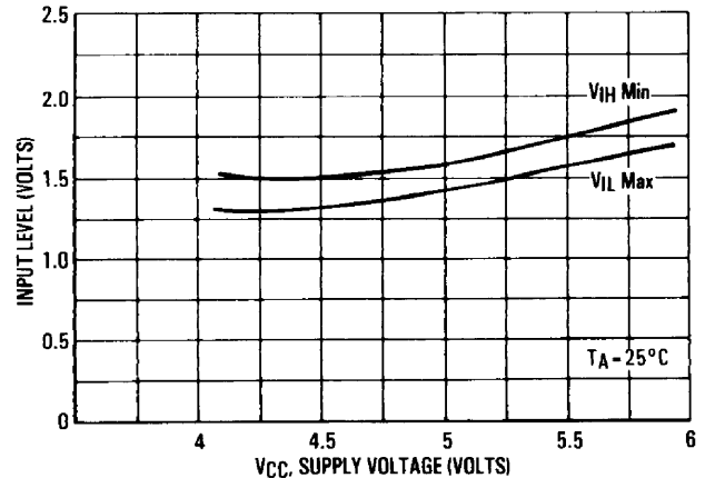
FIGURE 17 — DATA INPUT LEVEL versus SUPPLY VOLTAGE
