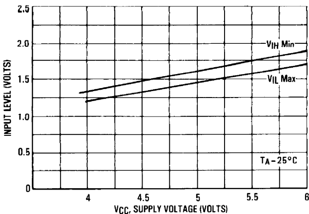
FIGURE 6 — \overline{\text{RAS}} , \overline{\text{W}} INPUT LEVEL versus SUPPLY VOLTAGE
