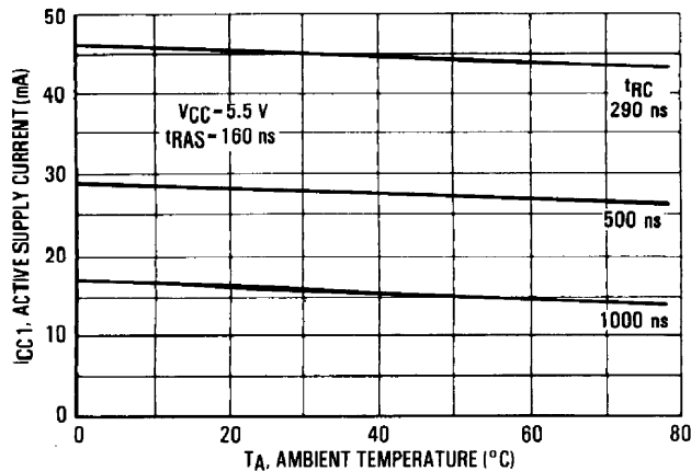
FIGURE 12 — I_{CC1} SUPPLY CURRENT versus AMBIENT TEMPERATURE (min t_{RAS} )
