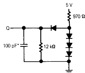
FIGURE 1 — OUTPUT LOAD
