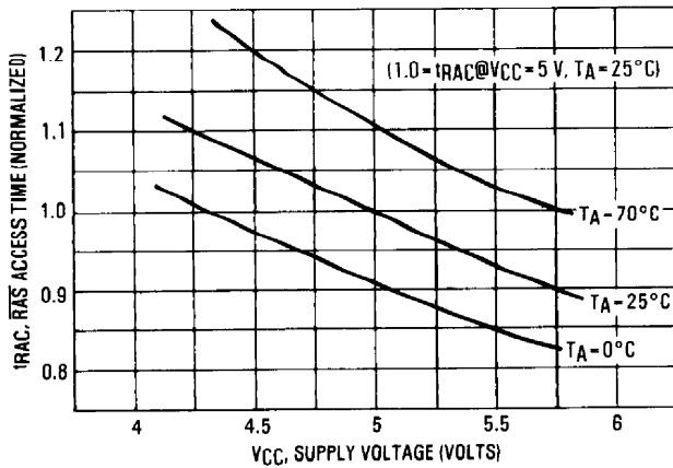
FIGURE 2 — \overline{\text{RAS}} ACCESS TIME versus SUPPLY VOLTAGE
