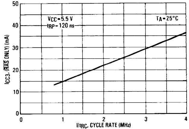
FIGURE 15 — I_{CC3} SUPPLY CURRENT versus CYCLE RATE
