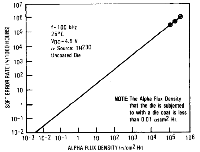
FIGURE 19 — SOFT ERROR RATE versus ALPHA FLUX DENSITY
