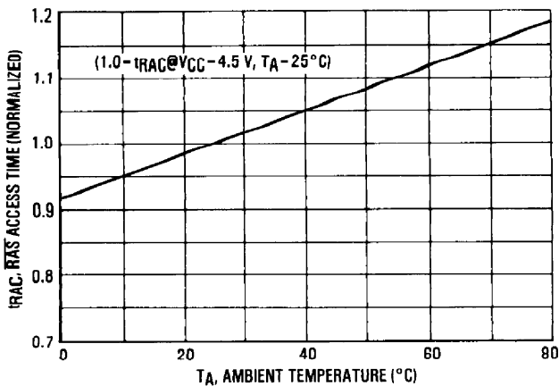
FIGURE 4 — \overline{\text{RAS}} ACCESS TIME versus AMBIENT TEMPERATURE
