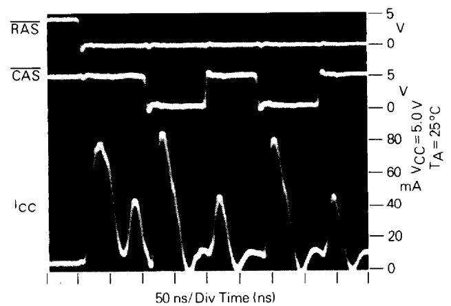
FIGURE 23 — PAGE MODE CYCLE
