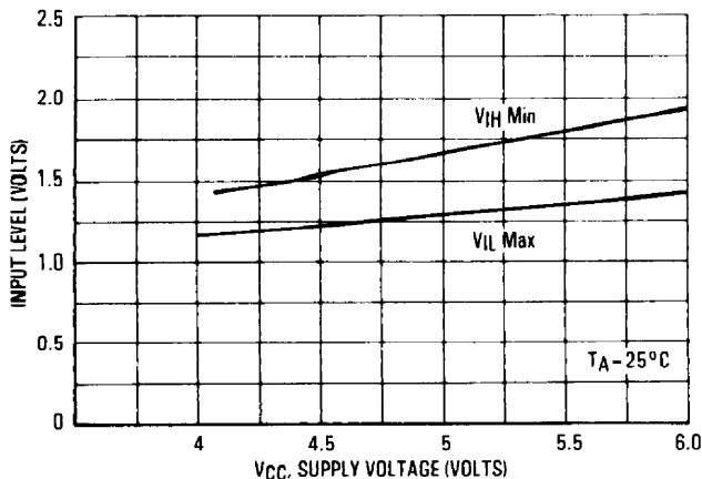
FIGURE 16 — ADDRESS INPUT LEVEL versus SUPPLY VOLTAGE
