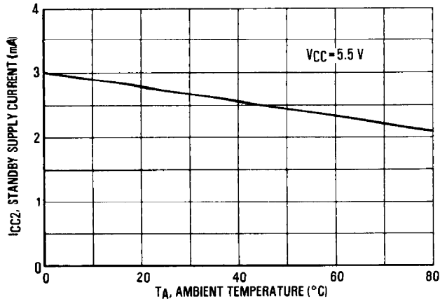
FIGURE 14 — I_{CC2} STANDBY CURRENT versus AMBIENT TEMPERATURE
