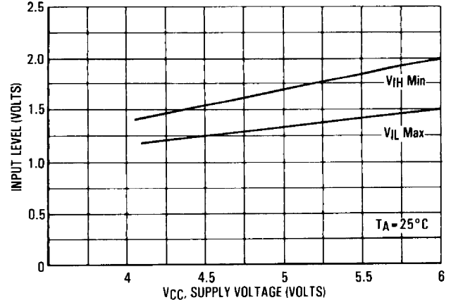
FIGURE 7 — \overline{\text{CAS}} , \overline{\text{W}} INPUT LEVEL versus SUPPLY VOLTAGE
